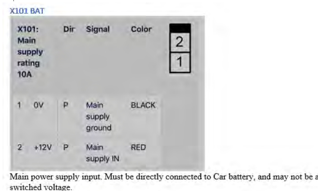
Figure 4.2 – X101 Powercable
